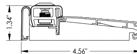
5 INSWING ADJUSTABLE THRESHOLD
