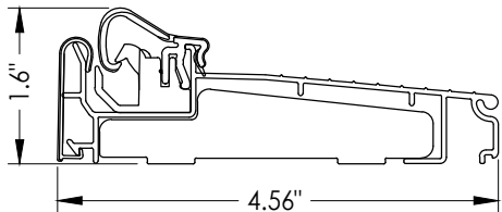
6 INSWING ARTICULATING THRESHOLD
