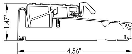
12 OUTSWING THRESHOLD
