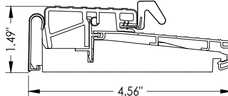
13 OUTSWING THRESHOLD
