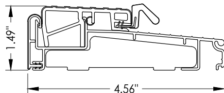
11 OUTSWING THRESHOLD
